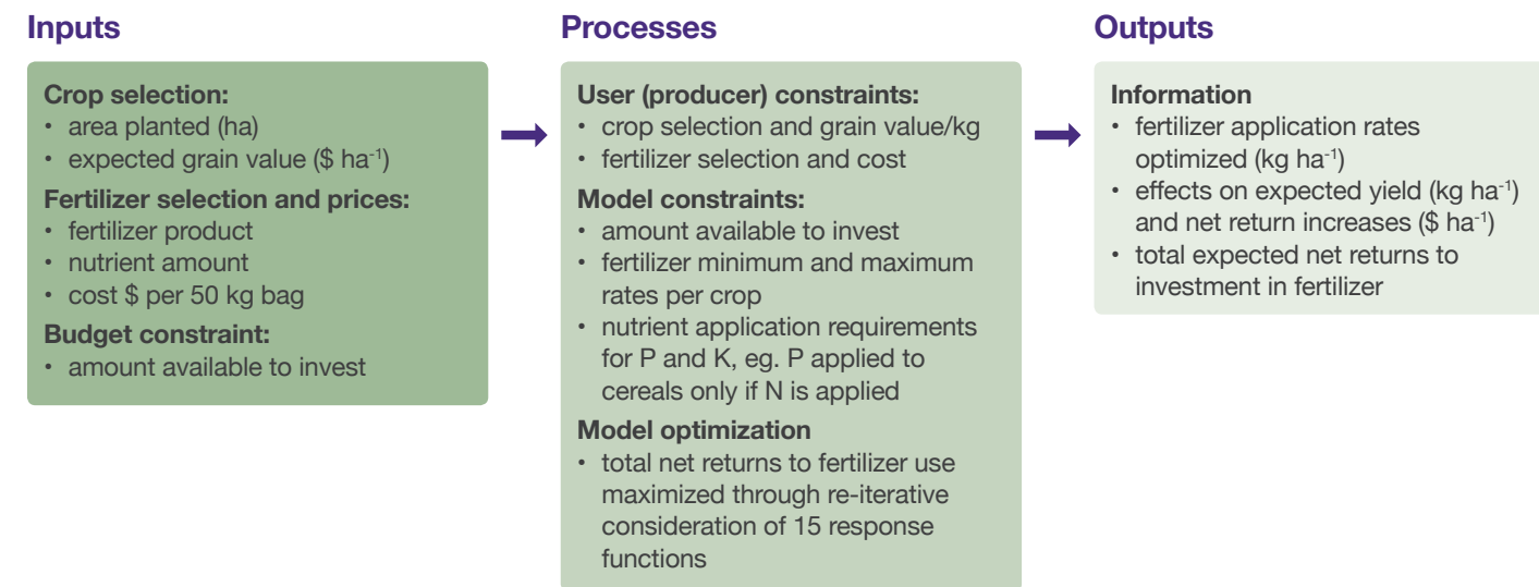
Figure 1: Operational flow model of the Fertilizer Optimization Tool (Source FOT Manual, 2014)
